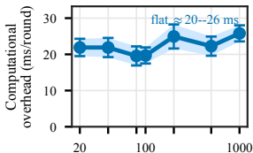
(b) Measured time
