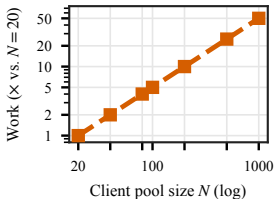
(c) Analytical work
