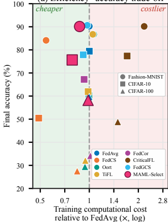
(a) Efficiency--accuracy trade-off
